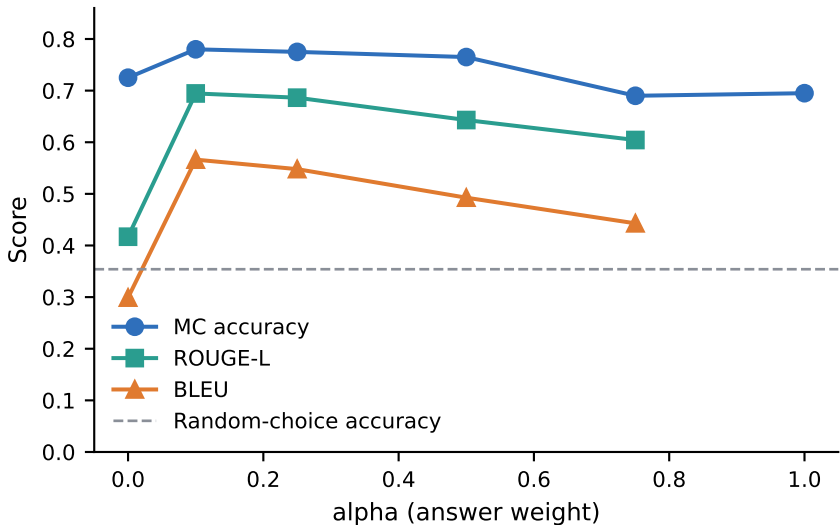
Explanation-aware alpha sweep
