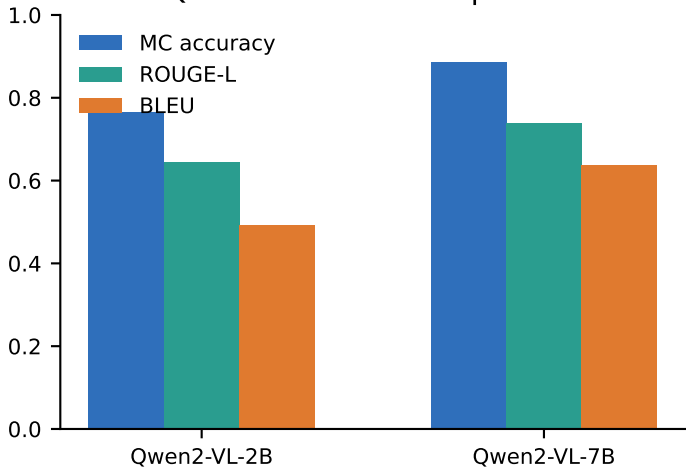
Qwen2-VL scale comparison
