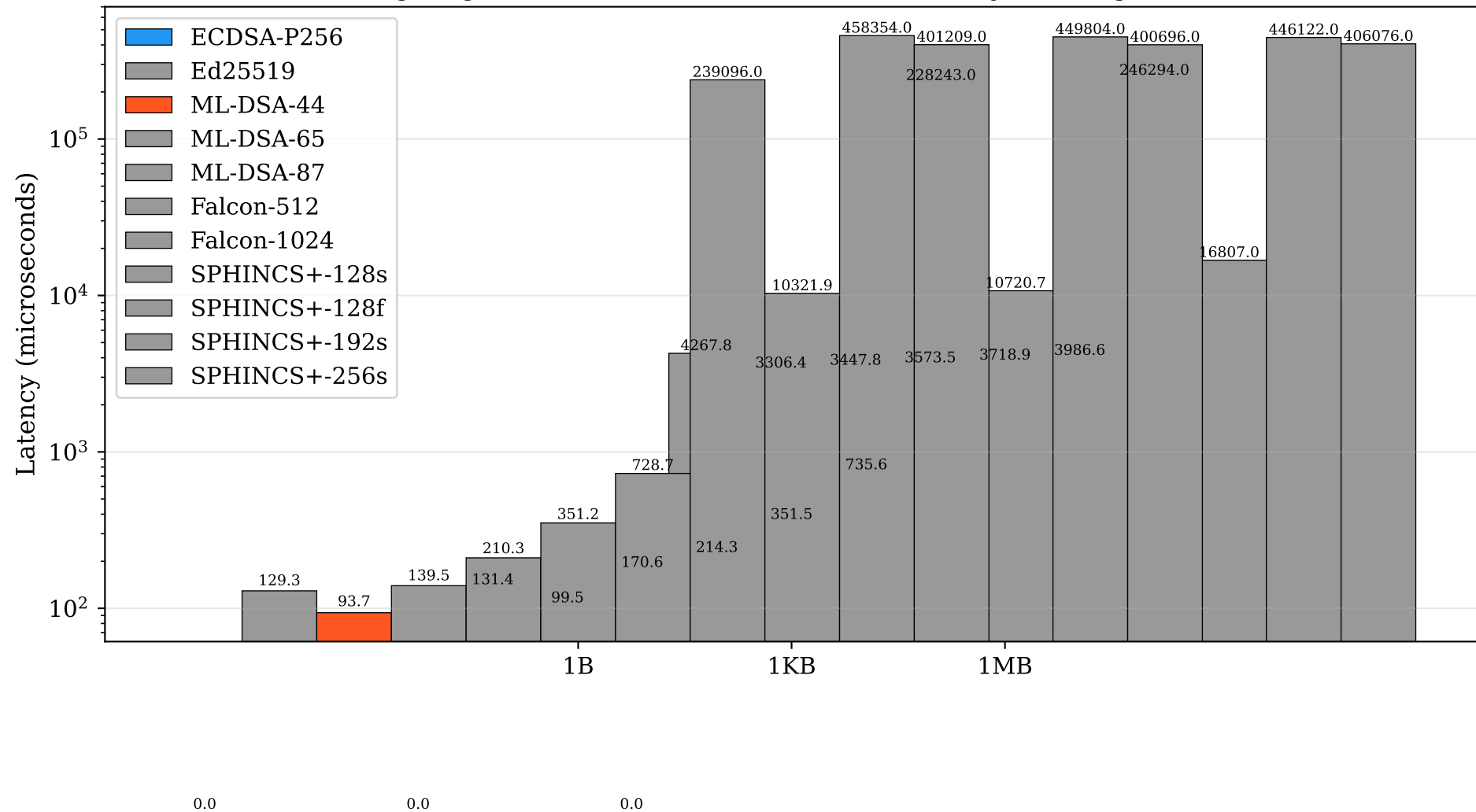
Signing Performance: The Quantum Tax by Message Size
