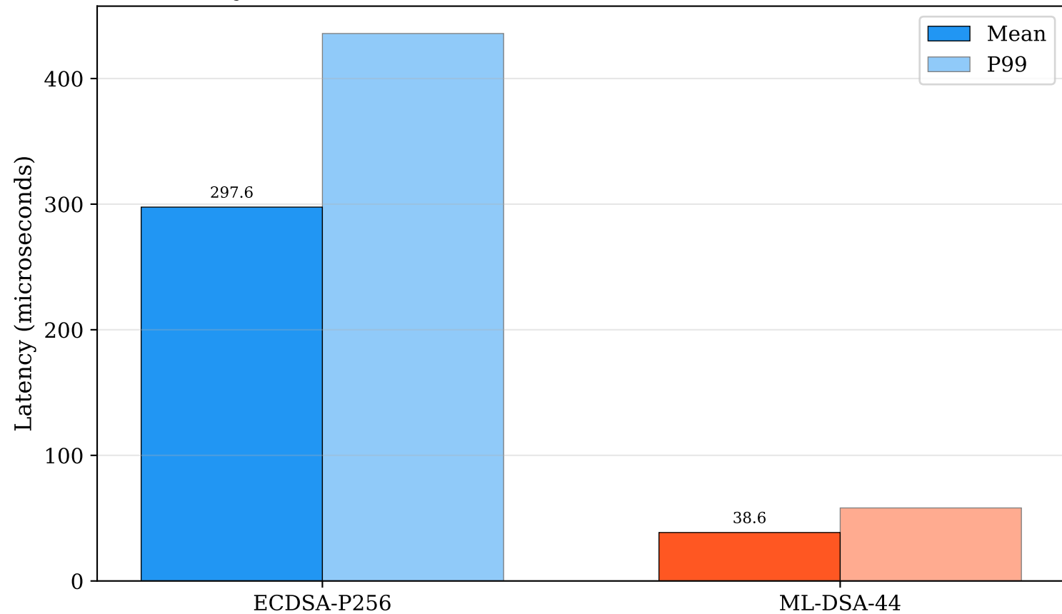
Key Generation Performance: Classical vs Post-Quantum
