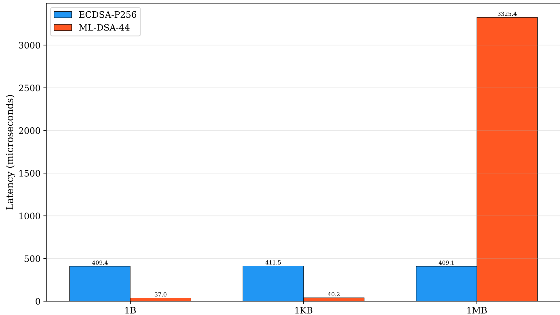
Verification Performance: The Verification Tax
