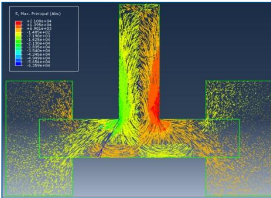
Fig 4 Tied Constraint
