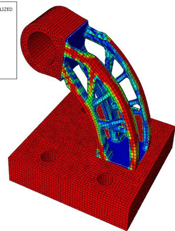
Fig 3 Entire Base Frozen
