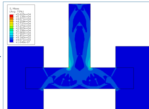
Fig 5 Von Mises Stress distribution in Optimization cycle 35
