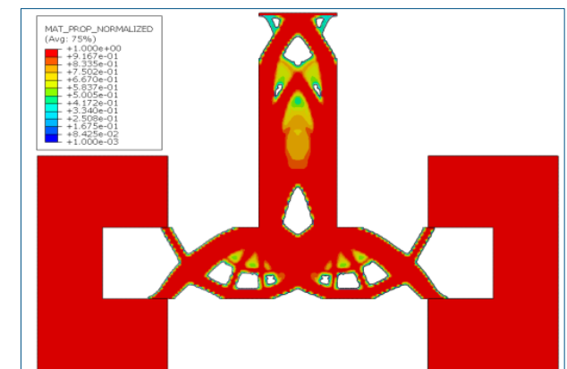
Fig 6 Iso density plot at 0.3 in cycle 35
