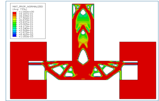
Fig 3 Iso density plot at 0.3 in cycle 67
