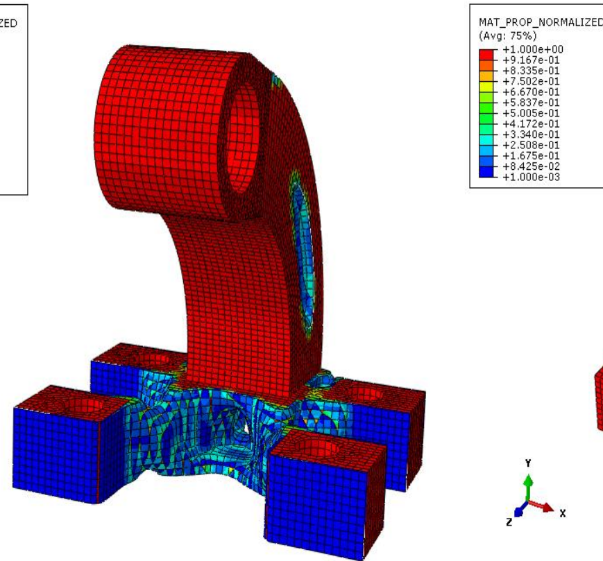
Fig 2 Only bolt hole regions are frozen
