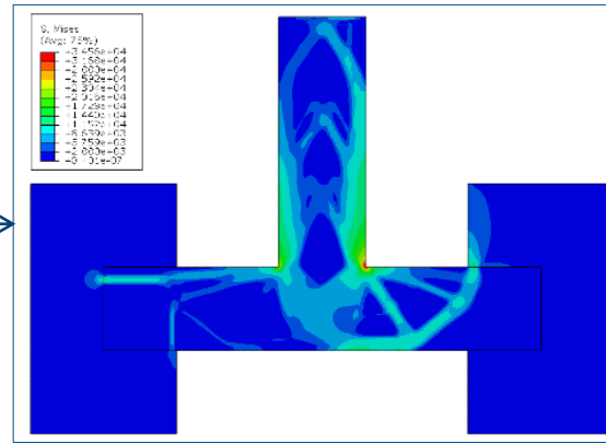
Fig 2 Von Mises Stress distribution in Optimization cycle 67
