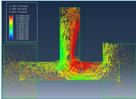
Fig 1 Nonlinear Contact
