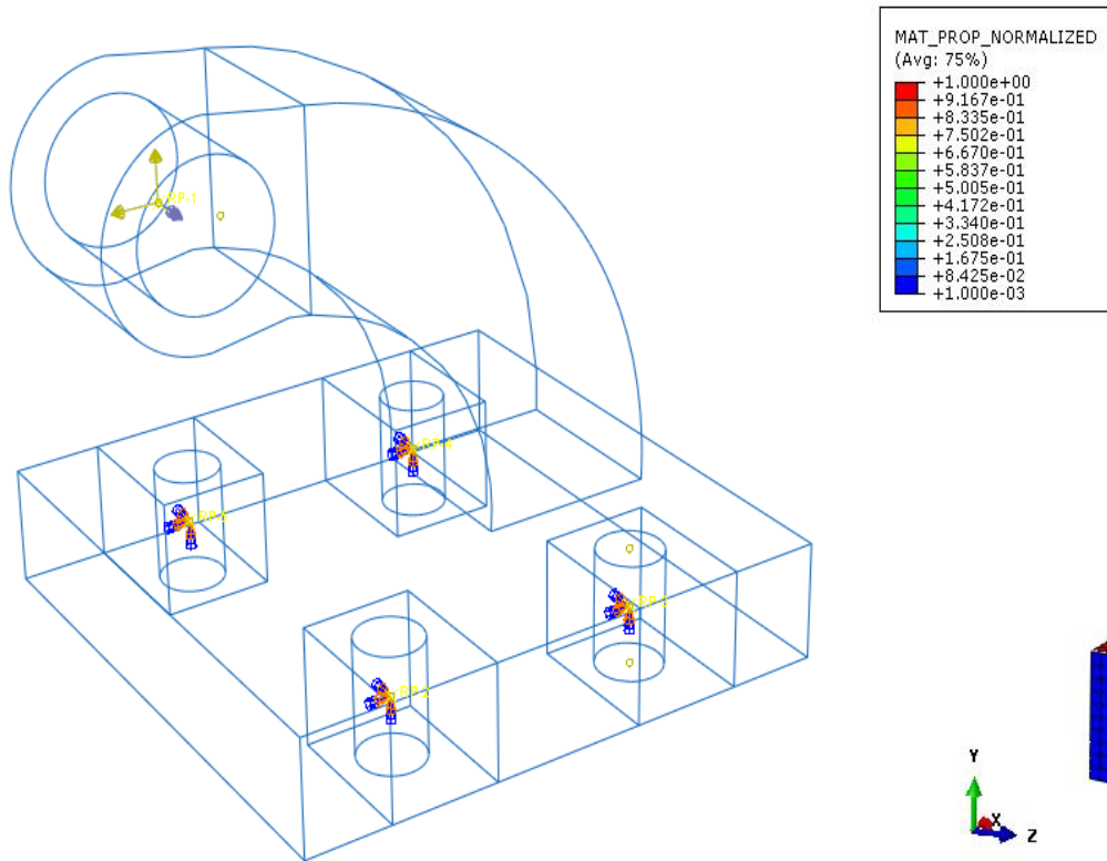
Fig 1 Loading and Boundary Conditions
