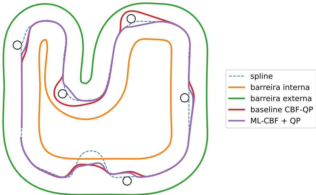
Pack6: baseline CBF-QP vs ML-CBF
