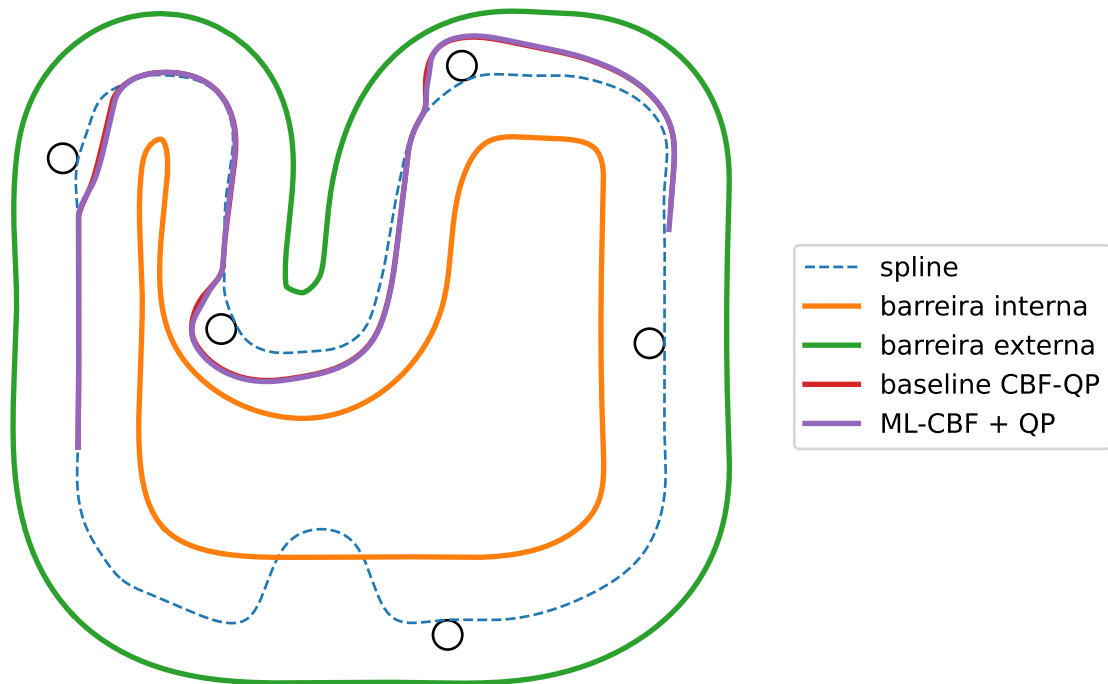
Pack5: baseline CBF-QP vs ML-CBF
