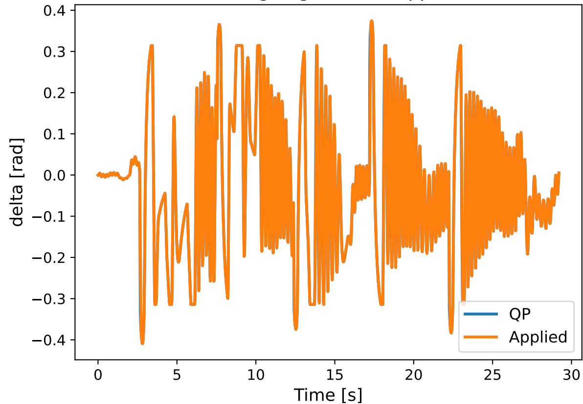
Steering angle: QP vs Applied
