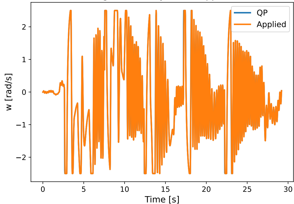
Angular velocity: QP vs Applied
