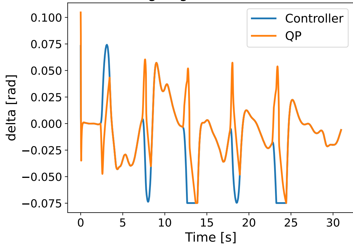
Steering angle: Controller vs QP
