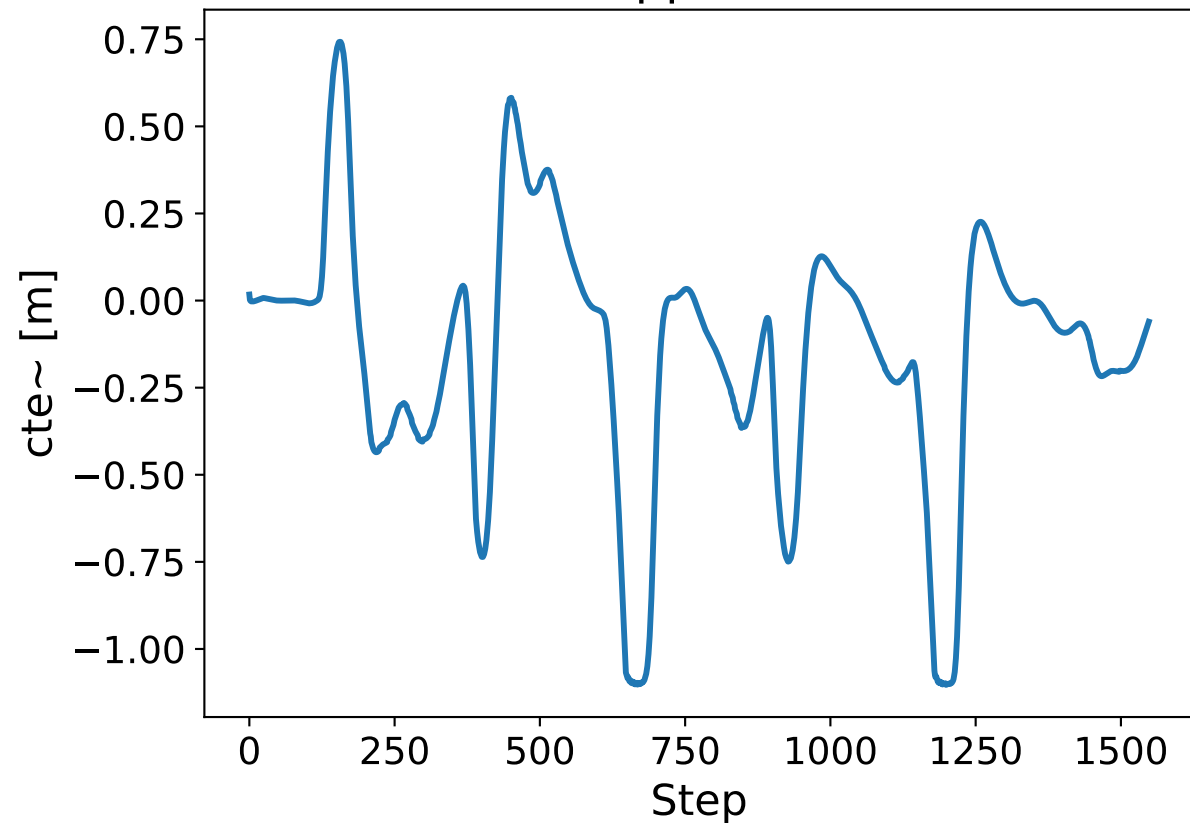
Lateral error (approx) - Pure Pursuit
