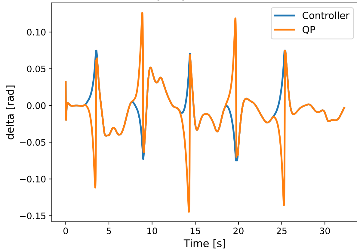
Steering angle: Controller vs QP
