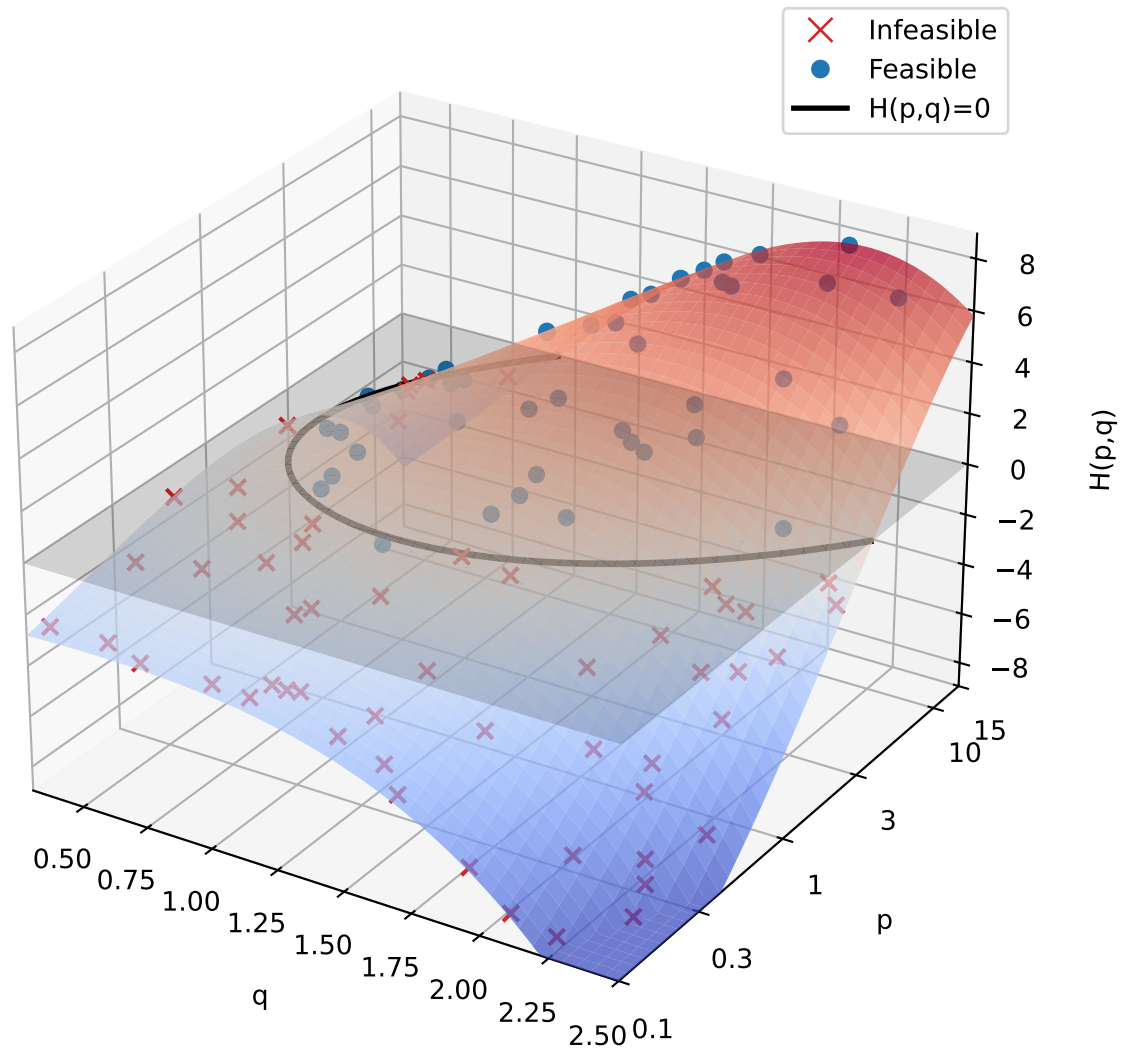
3D SVM feasibility function H(p,q) , degree 7
