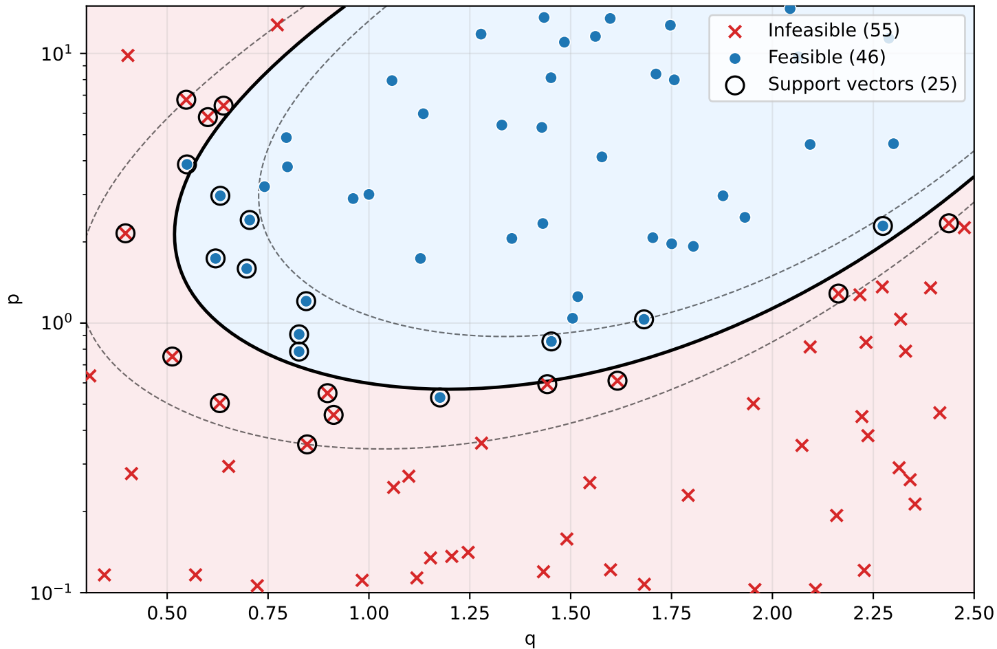
Polynomial-kernel SVM boundary, degree 7
