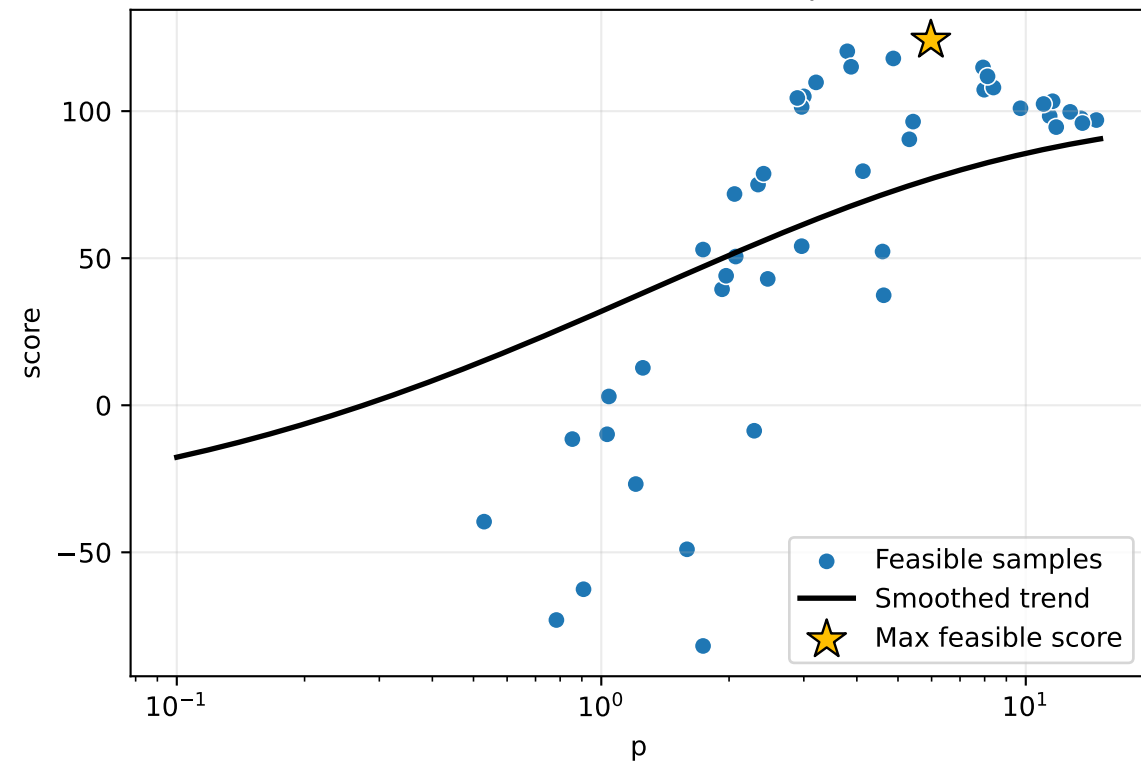
Score as a function of p
