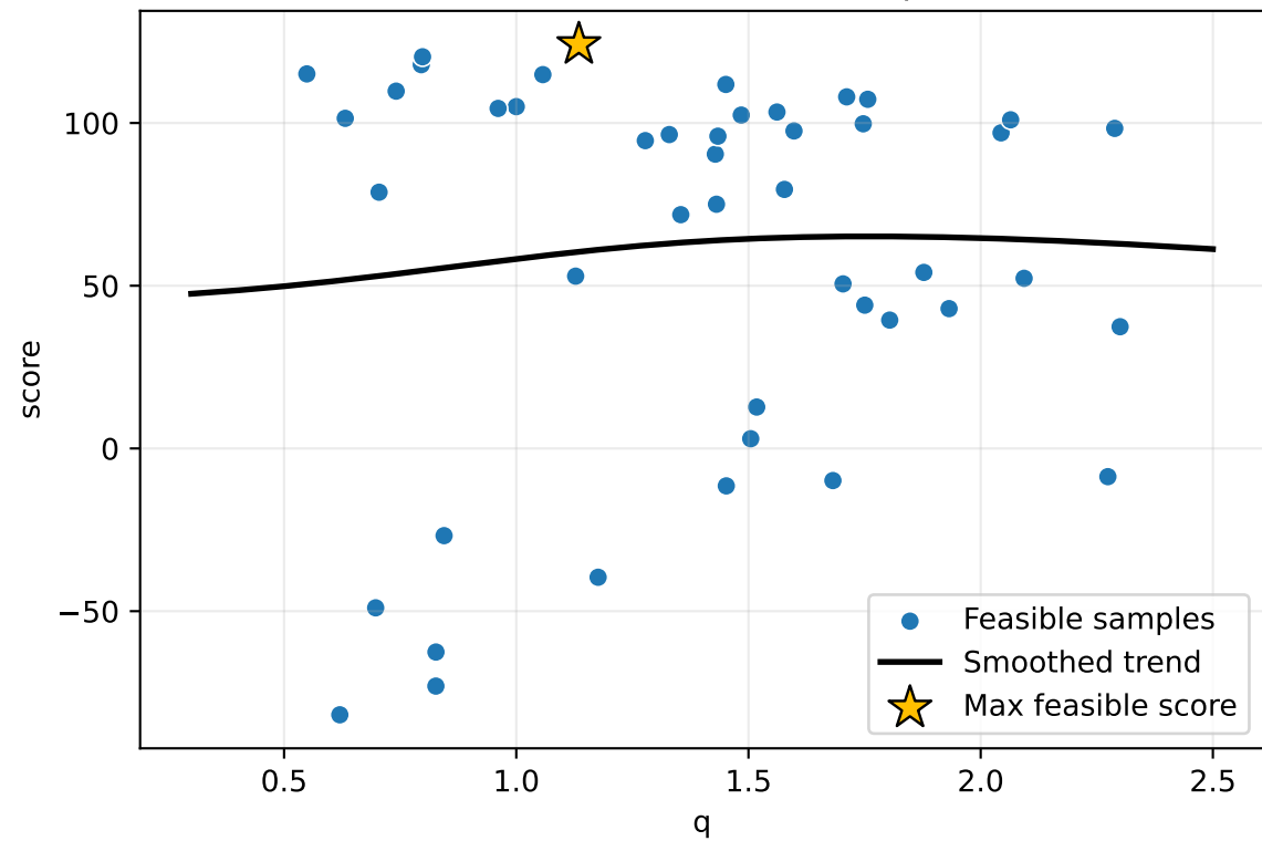
Score as a function of q
