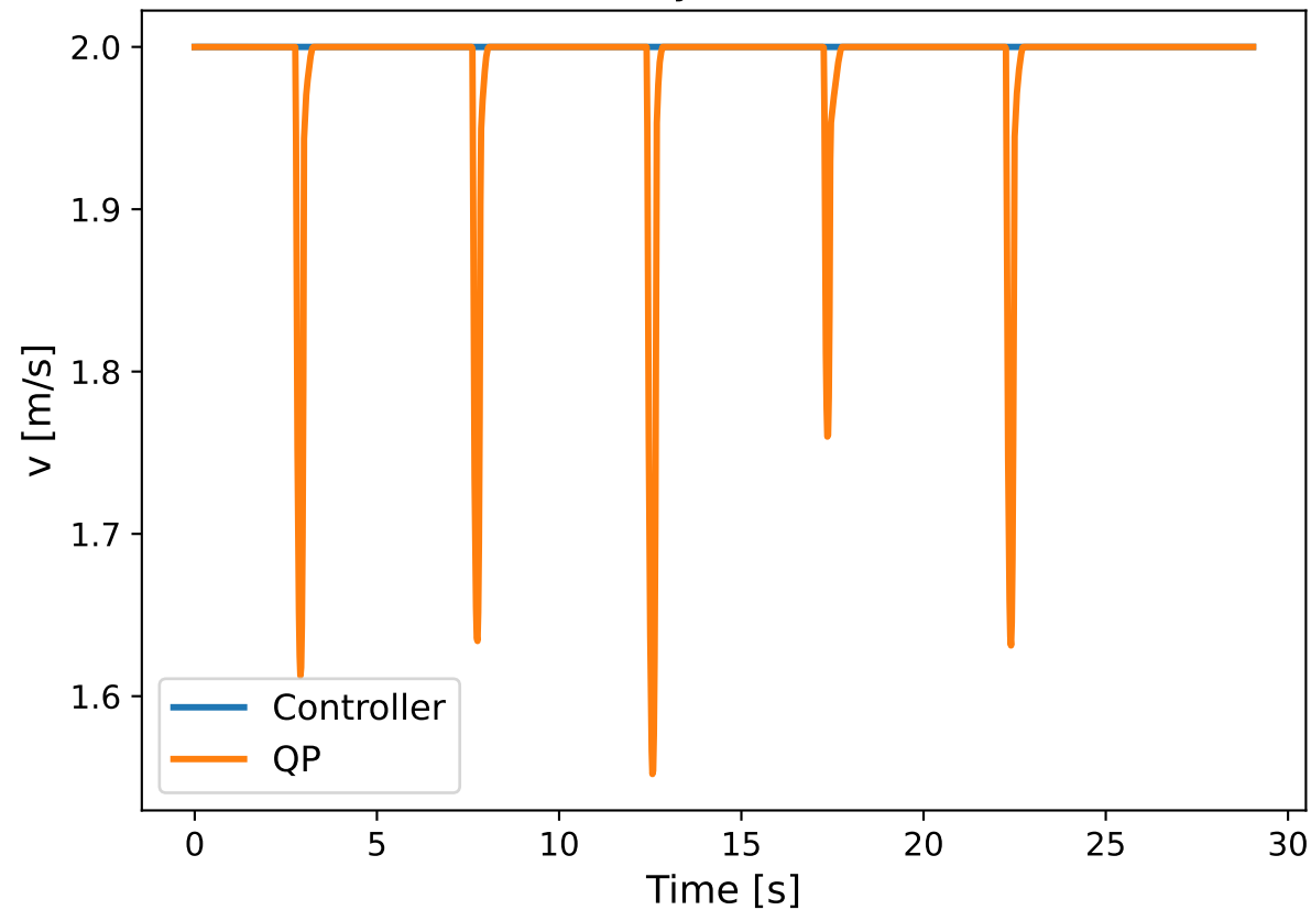
Linear velocity: Controller vs QP
