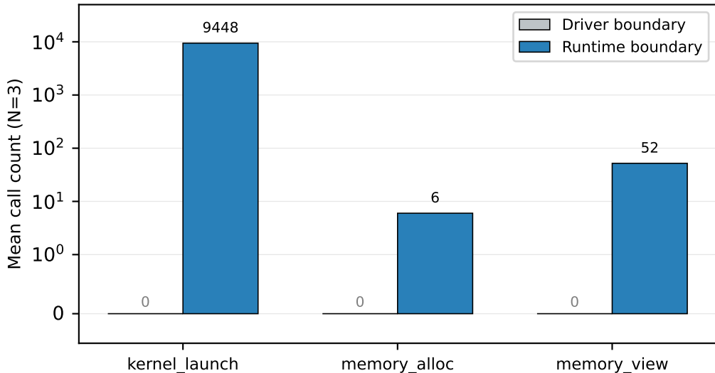
E1: Boundary Reachability on BI-V150
