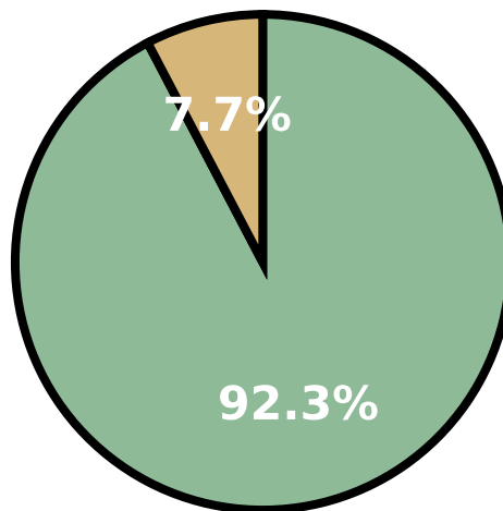
gemini-3-flash-preview (52)
