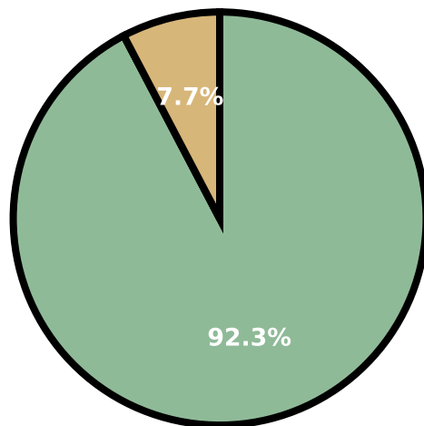
gemini-3-flash-preview
