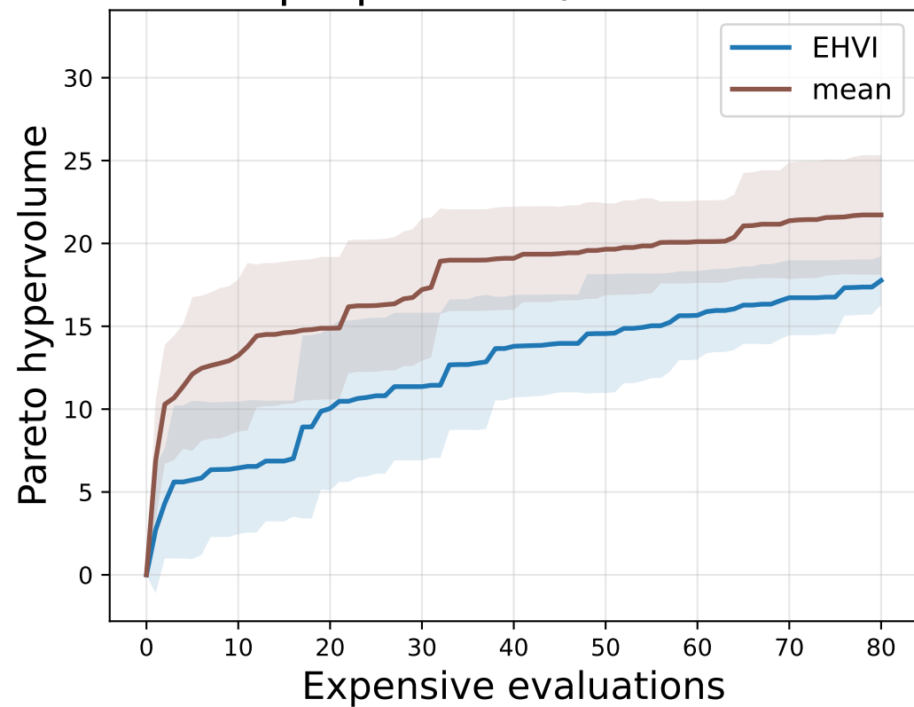
proposer16 / BoN16
