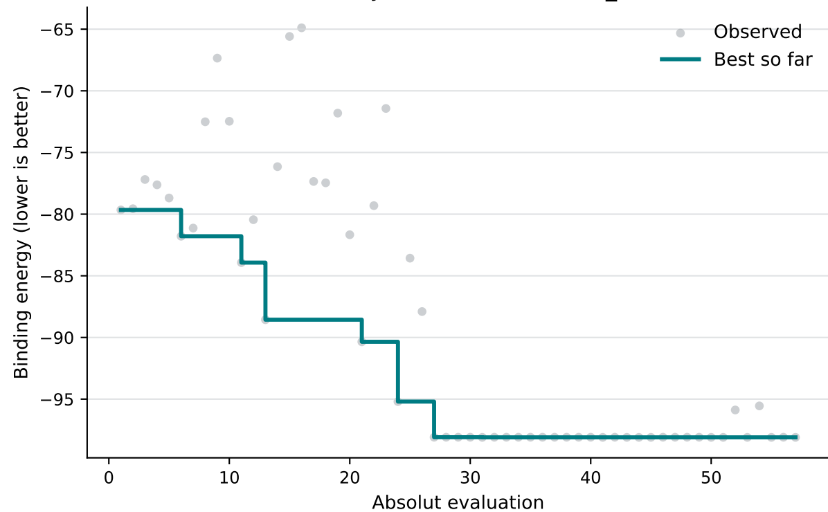
Antibody LDM: UCB on 1ADQ_A
