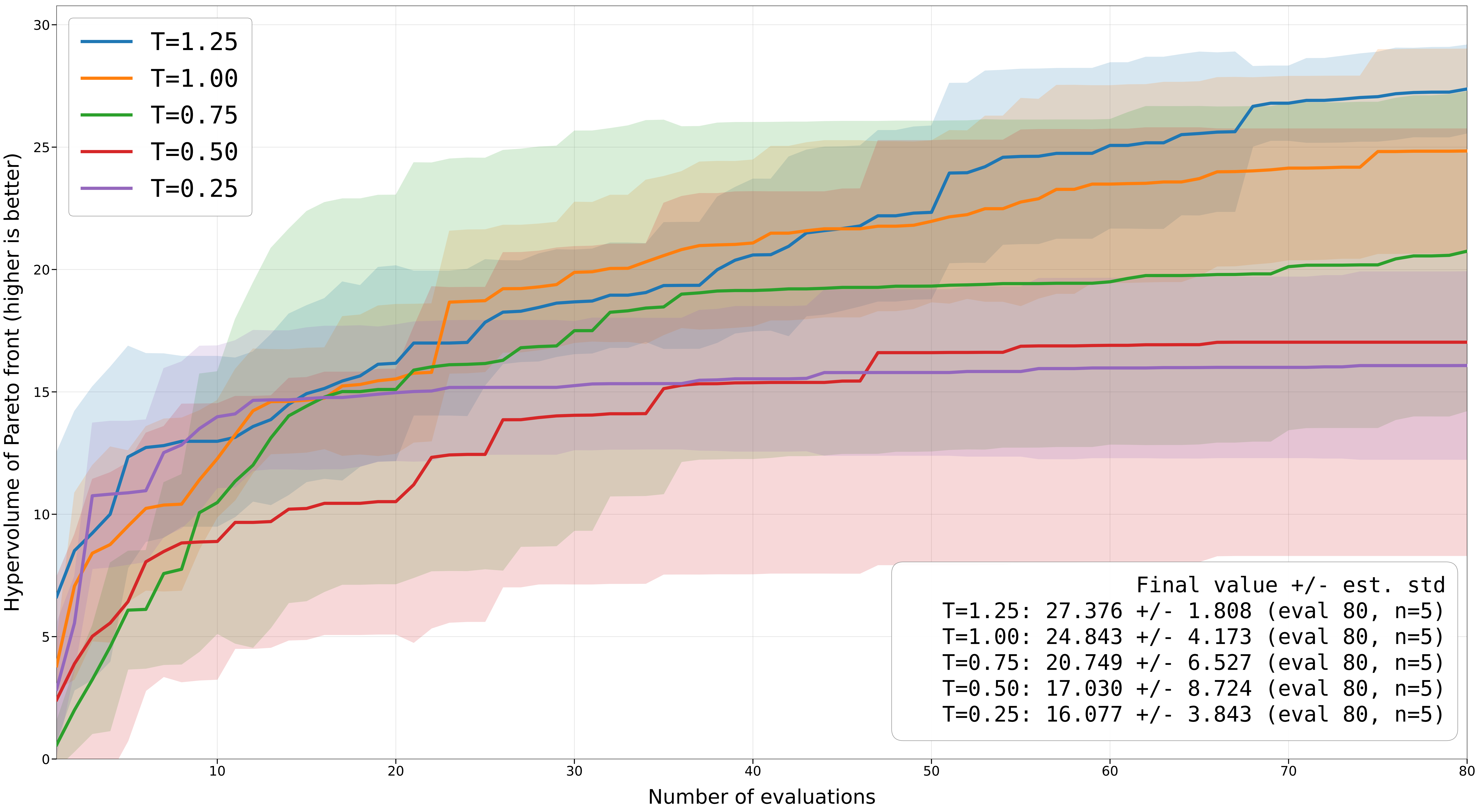
Temperature Sweep: Hypervolume by Number of Evaluations
