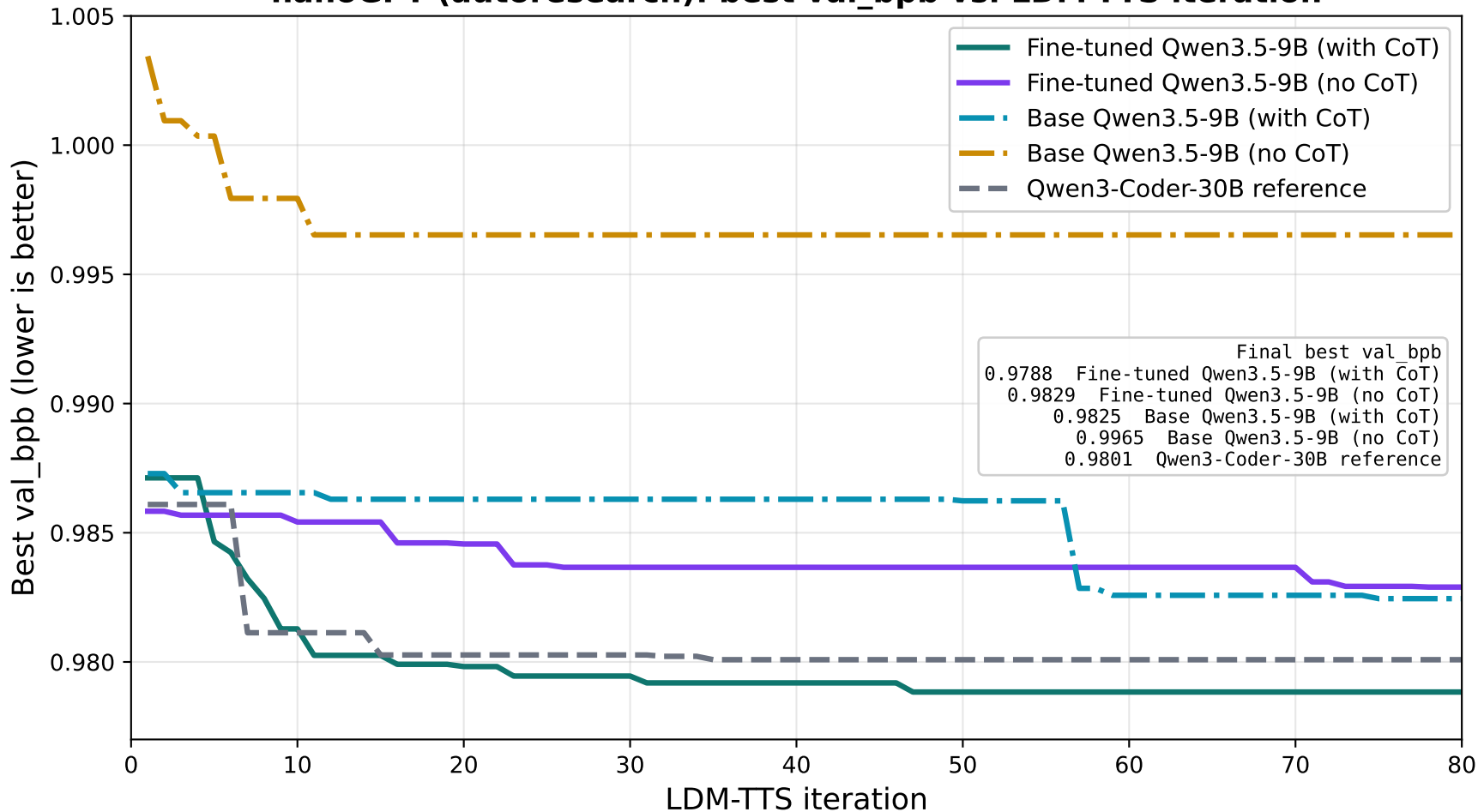
nanoGPT (autoresearch): best val_bpb vs. LDM-TTS iteration
