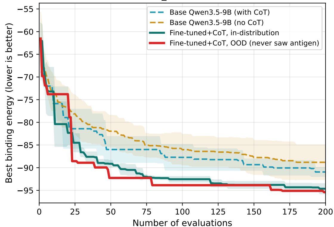
1H0D_C (held-out)
