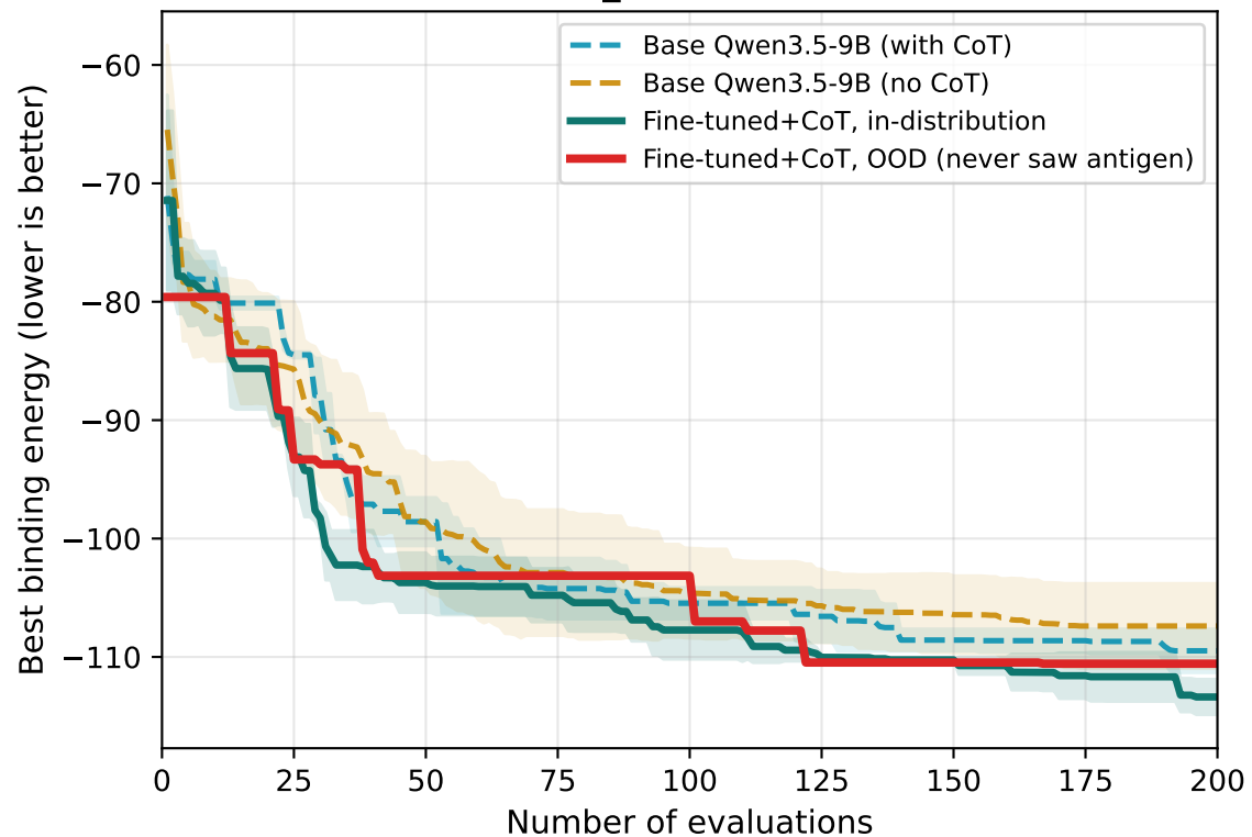
1FBI_X (held-out)
