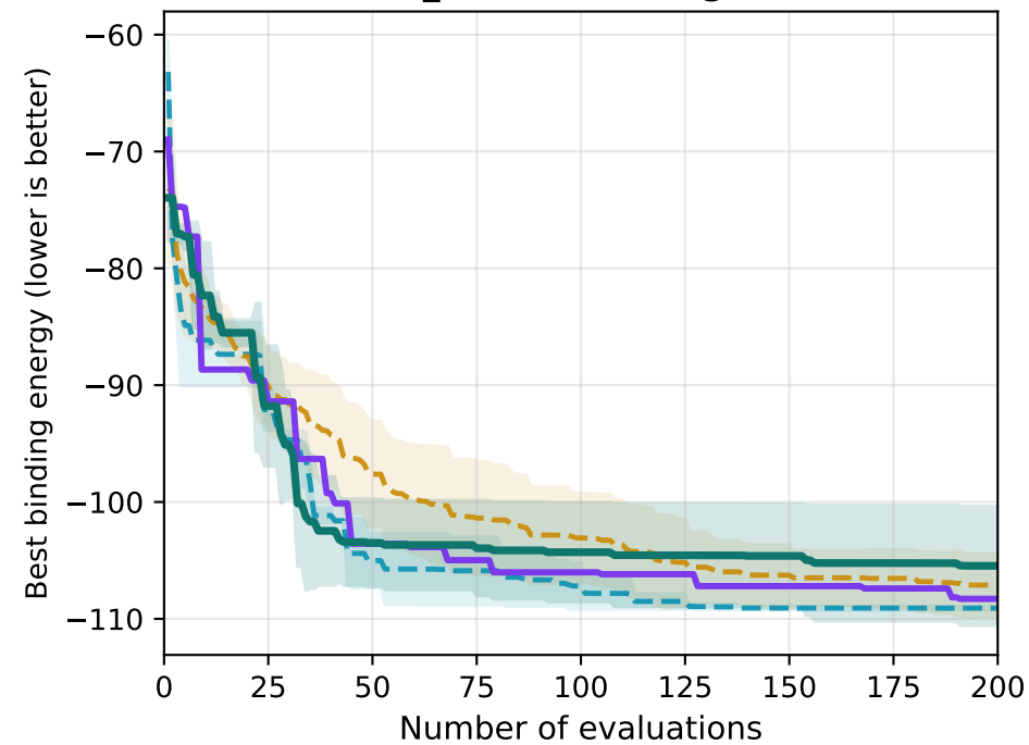
1OB1_C (CDRH3 length 11)
