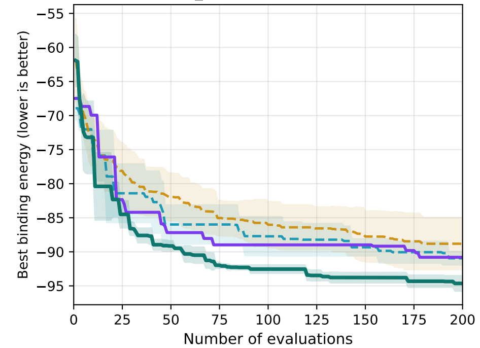
1H0D_C (CDRH3 length 11)
