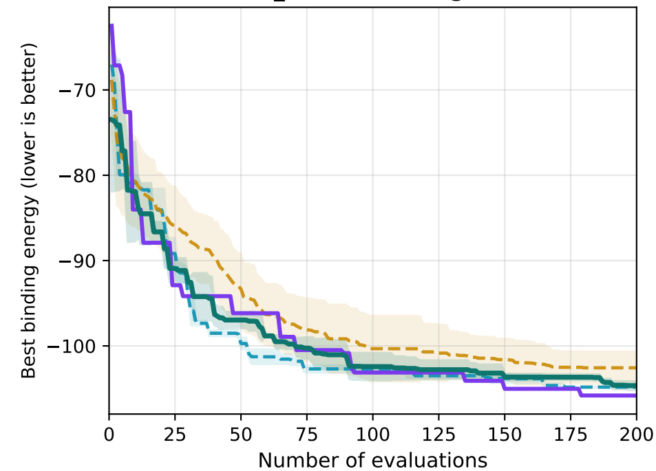
1NSN_S (CDRH3 length 11)
