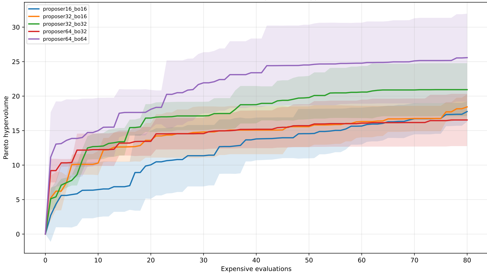
LDM-TTS (Qwen3.5-9B) for Molecular Design: Pareto Hypervolume Mean \pm Std
