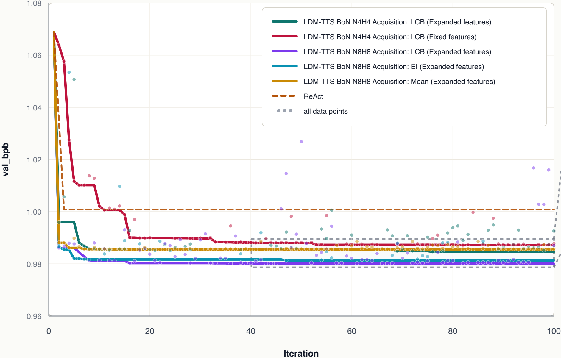
Best val_bpb by LDM-TTS (Qwen3-Coder-30B-A3B) iteration
