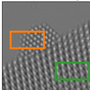
Blindspot denoising
