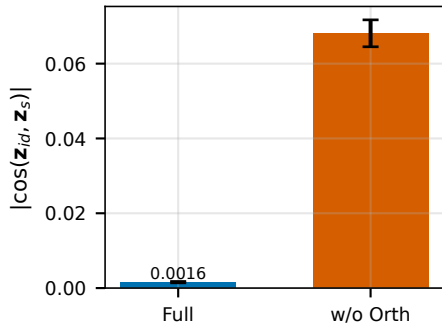
(a) Orthogonality (43x)
