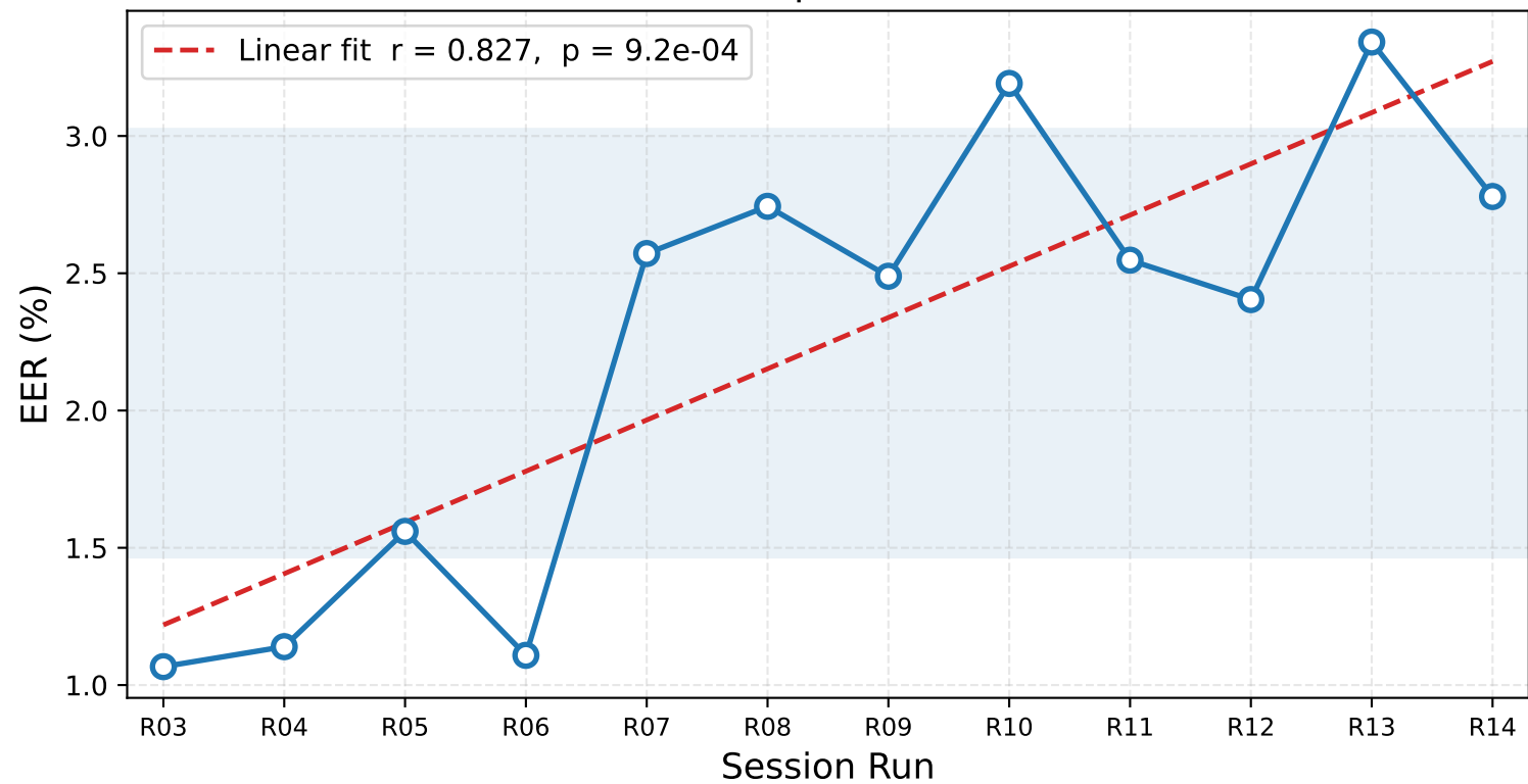
Per-Session EER: Temporal Drift (B2T Protocol)
