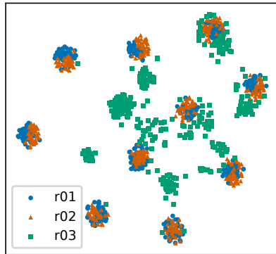
(b) BED z_{id} by session
