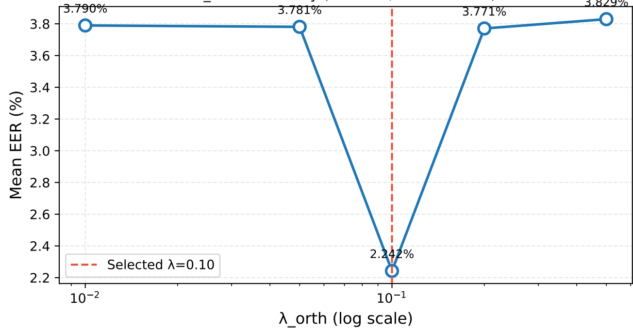
\lambda_{\text{orth}} Sensitivity (B2T EER, 2-seed mean)
