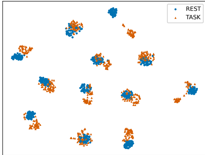
(b) z_{id} by state (co-located)
