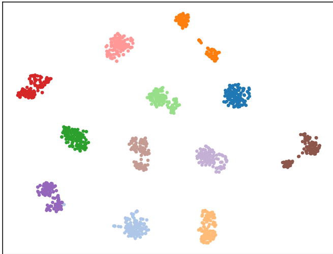
(a) z_{id} by subject
