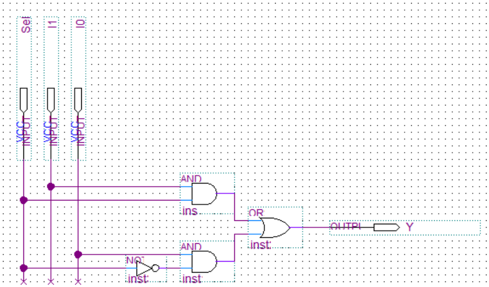
MUX2 1:
