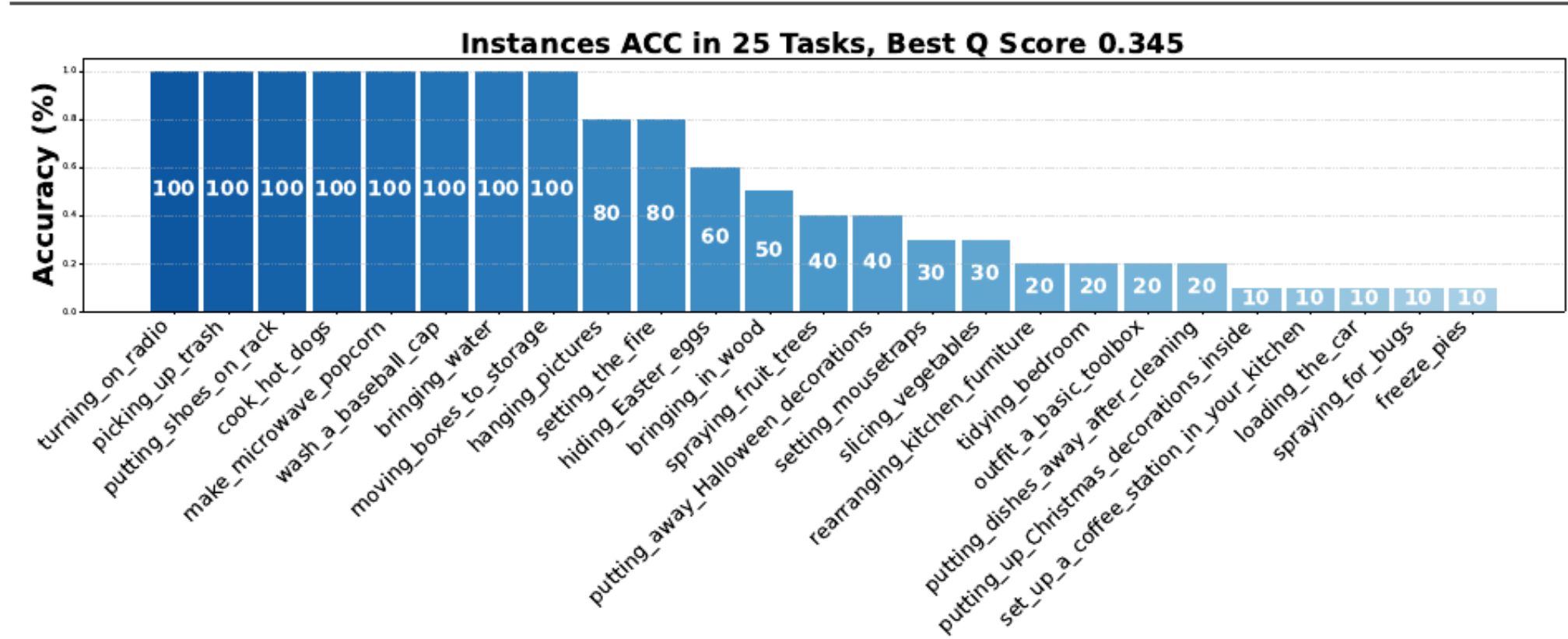
Figure 4: We can achieve an aggregated validation Q-score of 0.345 and a validation success rate of 15%
