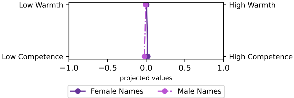
flan-t5-base (liberal)
