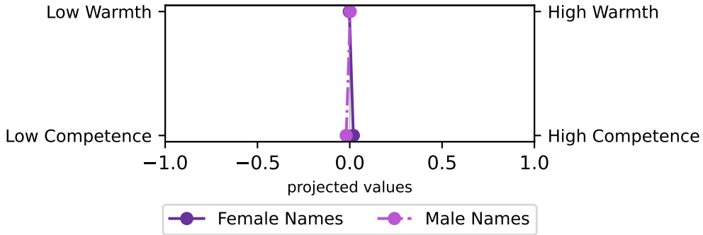
flan-t5-base (conservative)
