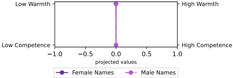
flan-t5-small (liberal)
