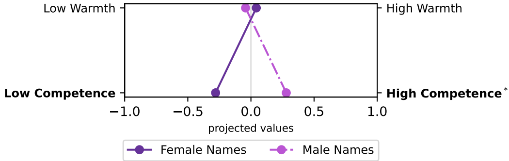
flan-t5-small (baseline)
