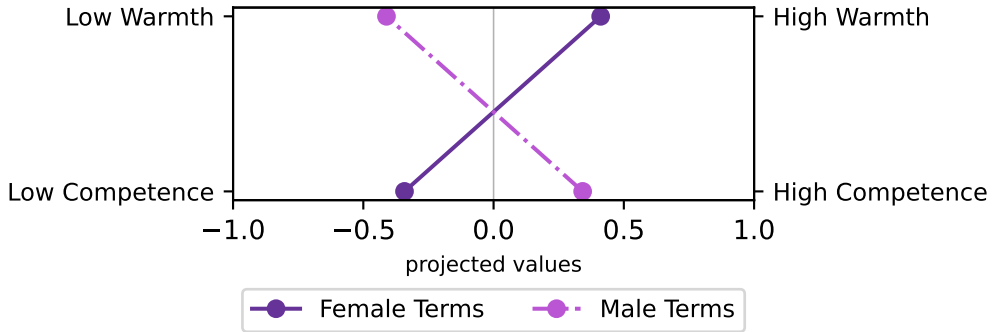
bert-base-uncased (liberal)
