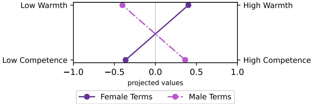
bert-base-uncased (baseline)
