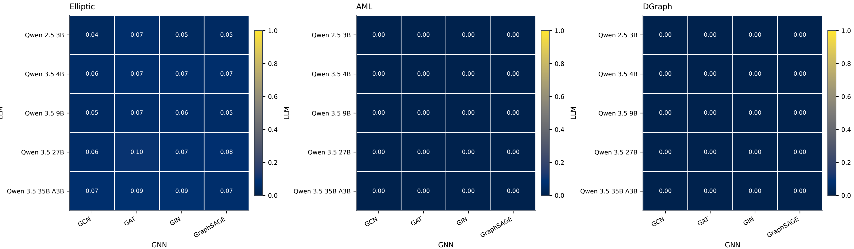
Fidelity F1 by dataset, GNN, and LLM
