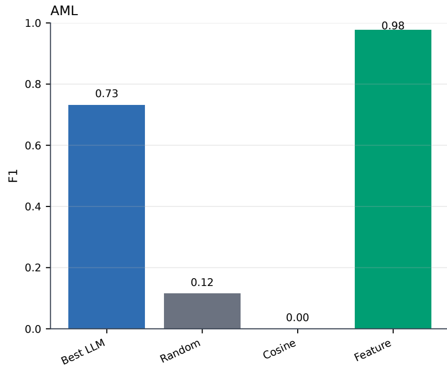
Best reconstruction F1 compared with baselines
