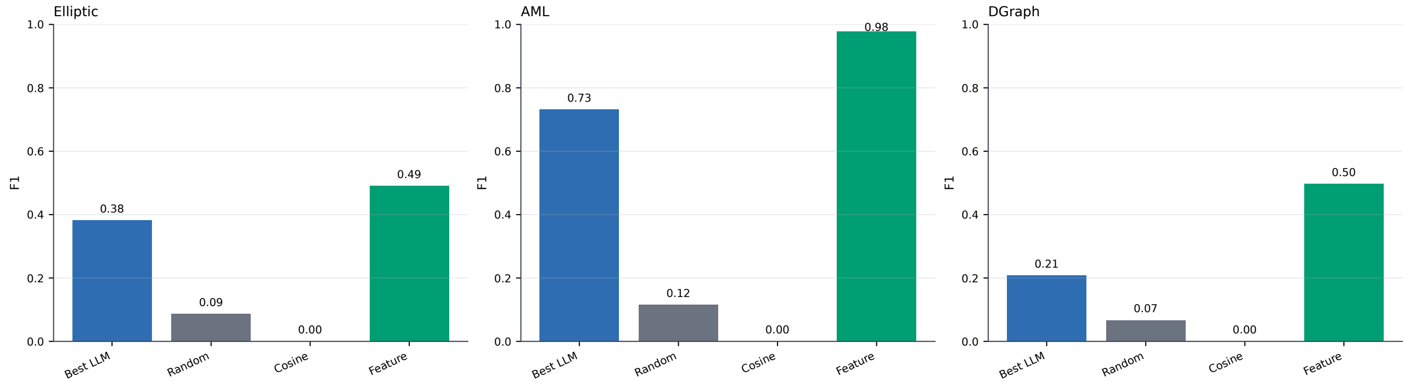
Best GNNExplainer-subgraph reconstruction F1 compared with baselines
