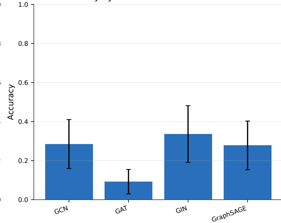
Mean accuracy by GNN
