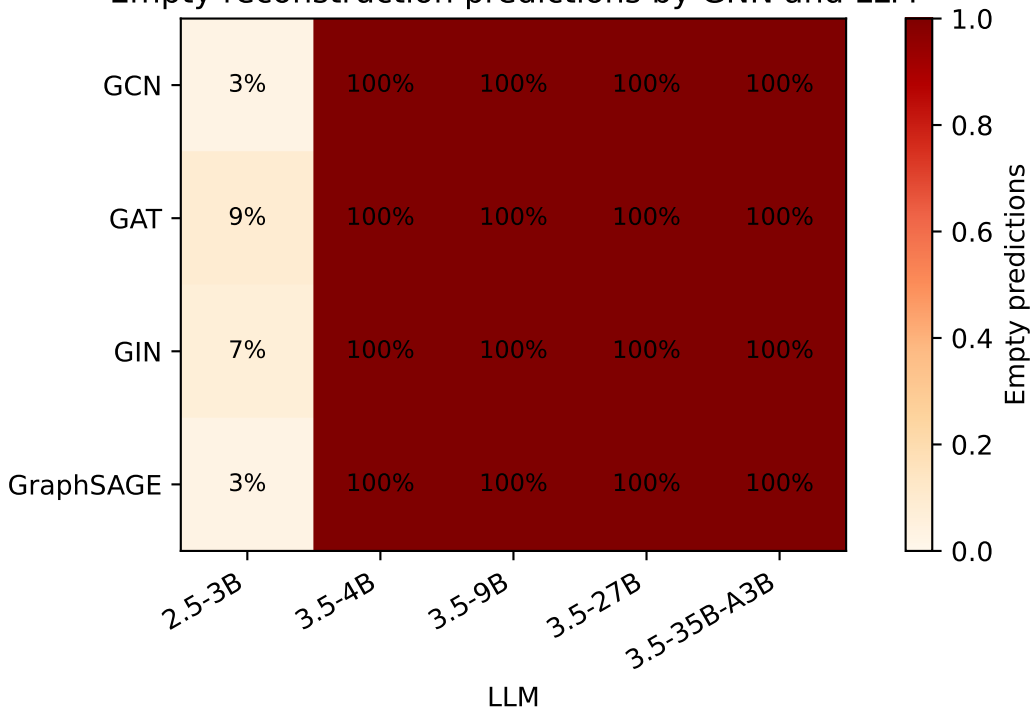
Empty reconstruction predictions by GNN and LLM
