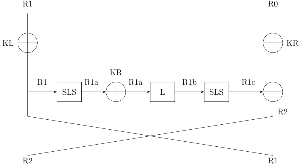
Figure 2: ITUbee MILP differential cryptanalysis sketch
