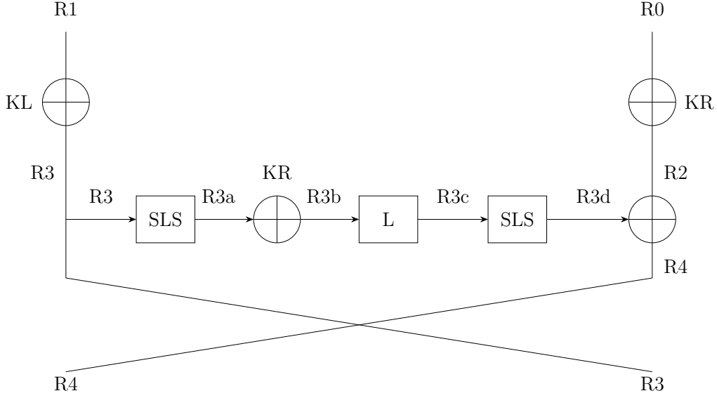
Figure 4: ITUbee MILP Related-Key Differential Cryptanalysis Sketch
