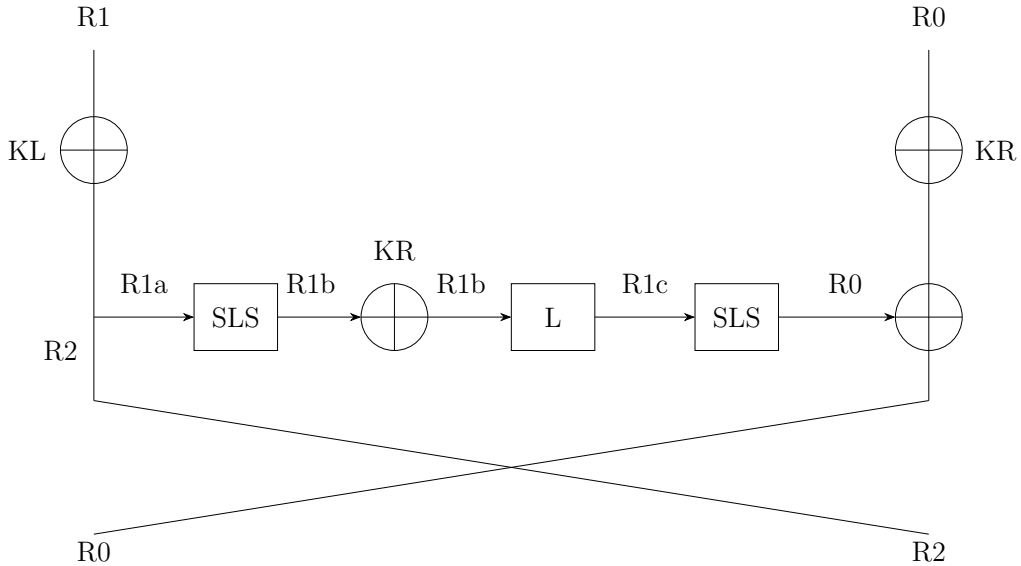
Figure 3: ITUbee MILP linear cryptanalysis sketch
