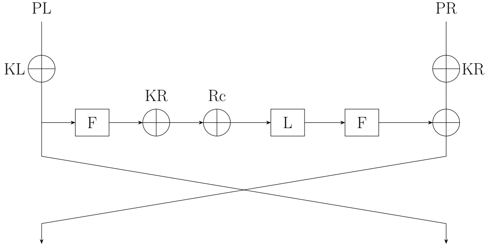
Figure 1: ITUbee round structure
