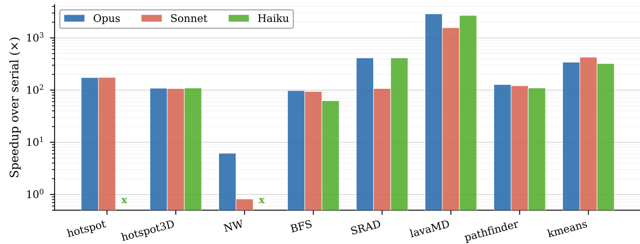
Best correct GPU kernel speedup per model (x = never produced correct output)
