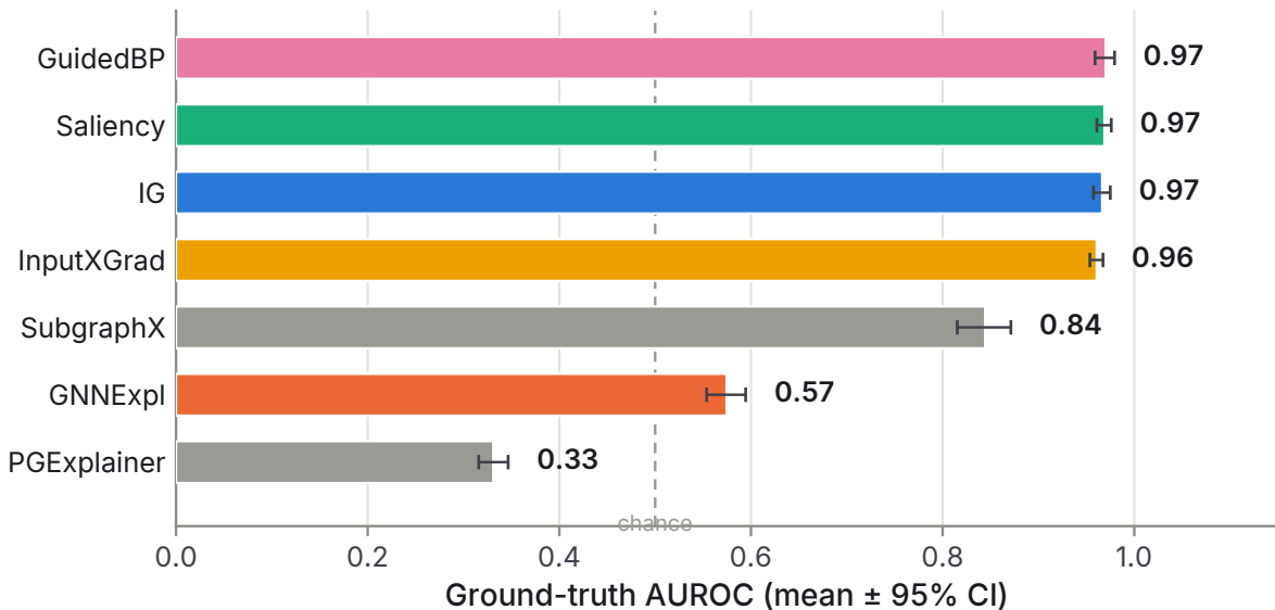
SynthMotifs · GINE · attribution vs ground truth · scaffold split
