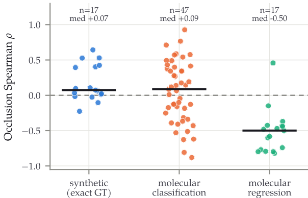
Faithfulness by task family
