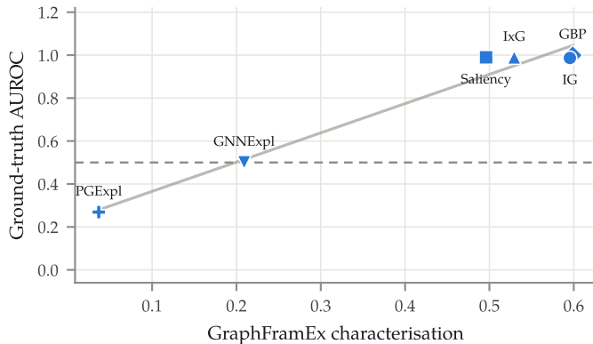
SynthMotifsXL · random · n = 120 \rho = +0.77 ( p = 0.072 )
