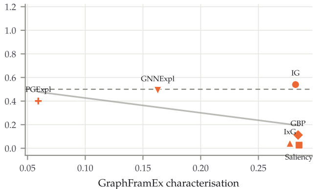
MUTAG · scaffold · n = 20 \rho = -0.49 ( p = 0.329 ) selects Saliency, truth says IG ( p < 0.001 )
