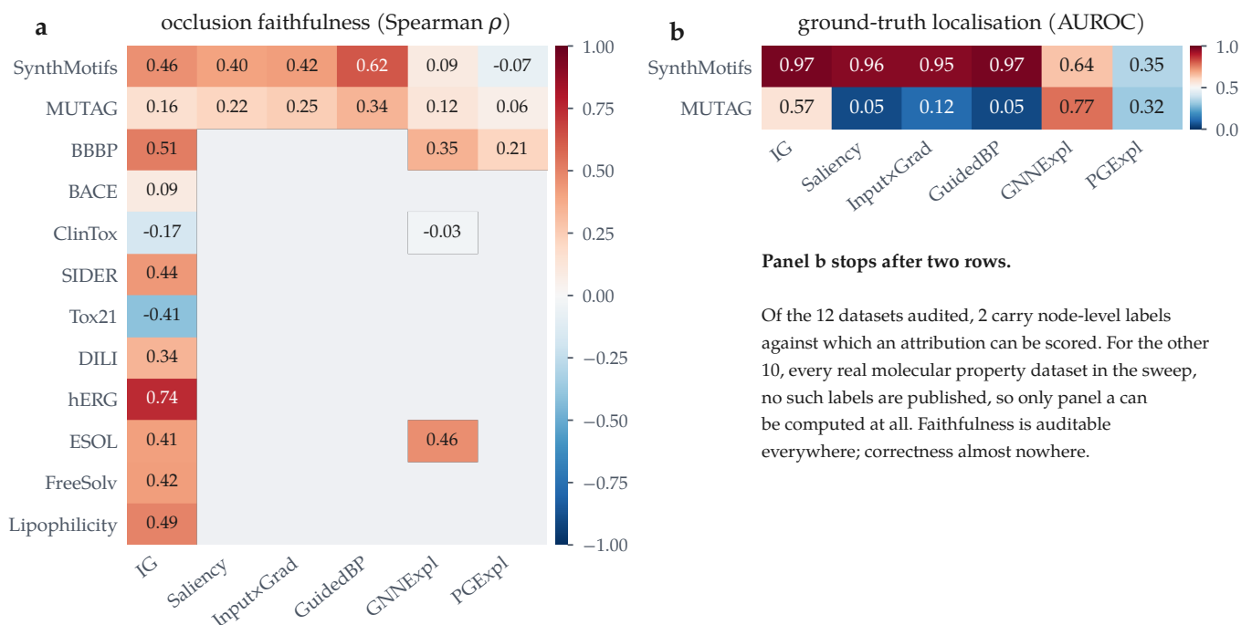
Figure 5: Reliability is a property of the (attributor, dataset) pair, not of the attributor. All committed GINE cells at the scaffold split. (a) Occlusion faithfulness over every audited dataset; blue = anti-faithful. (b) Ground-truth localisation, which exists for two datasets only. Panel b is short because correctness is unmeasurable elsewhere, not because it scores badly there: no molecular dataset in the sweep publishes per-atom labels. Blank cells were not audited; a thin outline marks a value carried from an earlier run.
