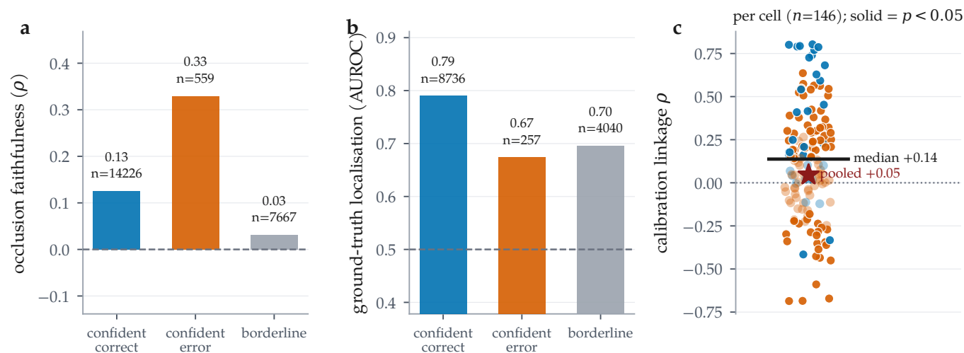
Figure 8: Regime stratification and calibration linkage, over the 26185 per-molecule audit records. (a) Occlusion faithfulness and (b) ground-truth localisation by confidence/correctness regime; n is printed per bar because ground truth exists for only a minority of molecules. Localisation on confident-error molecules degrades (0.790 to 0.674, n = 257 ) while occlusion faithfulness on the same molecules improves (0.126 to 0.330). (c) Calibration linkage computed per cell (solid = p < 0.05 ): the median cell is clearly positive, but pooling all molecules into one correlation attenuates it to near zero, a Simpson’s paradox and a caution against reporting the pooled number.
