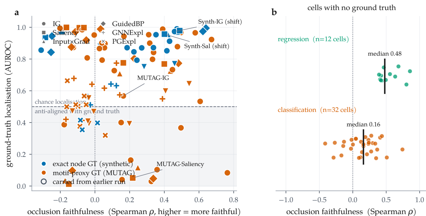
Figure 2: The two axes come apart, and for most cells only one of them exists. (a) Every committed cell carrying a node-level ground truth ( n = 114 ), plotted as occlusion faithfulness against ground-truth localisation; colour distinguishes exact synthetic ground truth from the MUTAG motif proxy, marker distinguishes attributor, and open markers are rows carried from an earlier run. The shaded band is GT AUROC < 0.5 : attributions there are anti-aligned with the true motif. 13 cells sit in the lower-right region, positively faithful to the model and anti-aligned with the truth. (b) The remaining 44 combinations, on real molecular datasets, have no published per-atom labels: only the horizontal axis is measurable for them.
