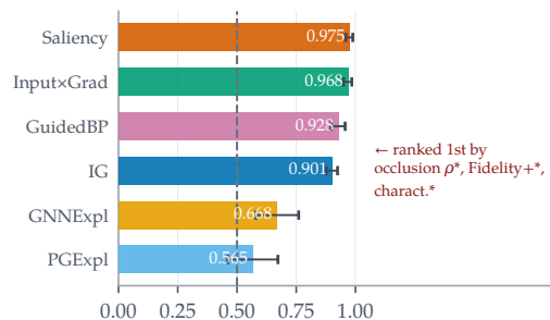
SynthMotifs-GINE: scaffold shift, n=20
