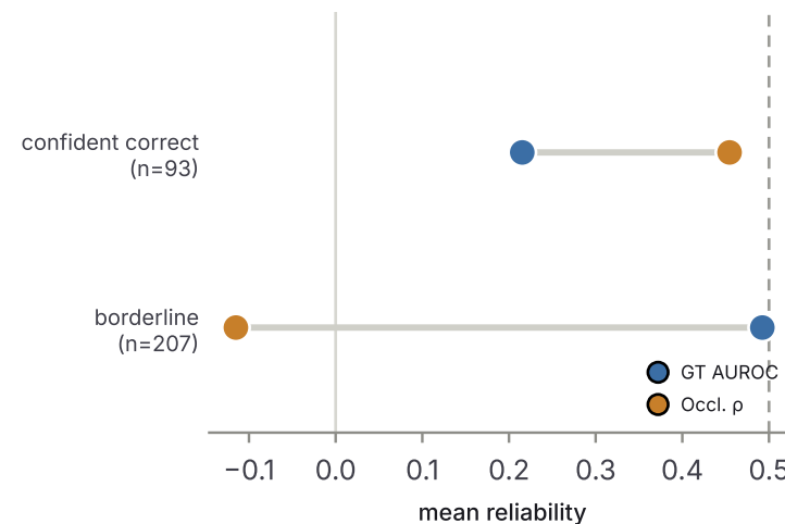
f reliability by regime (pooled)
